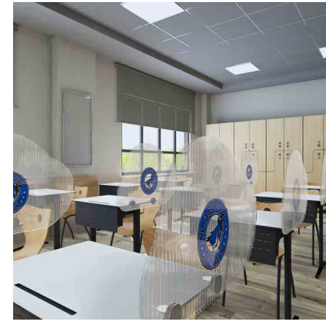
CUMULUS (B OPTION) DIMENSION - 2'-7.5" W X 1'-10" H MATERIAL - DIGITALLY PRINTED ACRYLIC, METAL
