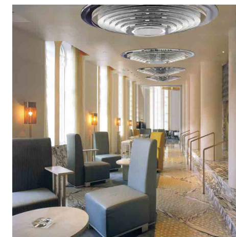
CENTRIC DIMENSION - Ø3'-11" X 6" PER ELEMENT MATERIAL - ACRYLIC, ALUMINUM LIGHTING - LED
